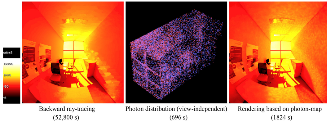
Fig. 2. Example processing time and typical sampling artefacts with a data-driven model (Laser Cut Panel (LCP) in the upper window zone) by backward ray-tracing with irradiance cache (left) and photon-mapping (center and right) [59]. The former has problems to resolve caustics (e.g. the LCP's deflection to the ceiling) and produces artefacts where the BSDF is not sufficiently sampled (e.g., along the wall). Photon-mapping relies on the rapid forward distribution of photons and avoids problems of backward ray-tracing but produces typical noise artifacts where the photon density is low (e.g., on the desk in the foreground). Source: HSLU.
