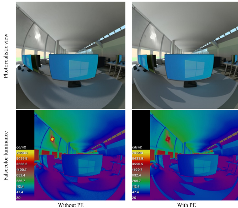
Fig. 3. Simulation without (left) and with (right) peak extraction (PE) from the high resolution BSDF data (max. 4096x4096). Note the differences in the sharpness of the shadow patterns and the size and luminance of the sun patch. The maximum luminance is 163,000 \text{cd/m}^2 (left) and 4,260,000 \text{cd/m}^2 (right). Source: Bartenbach.
