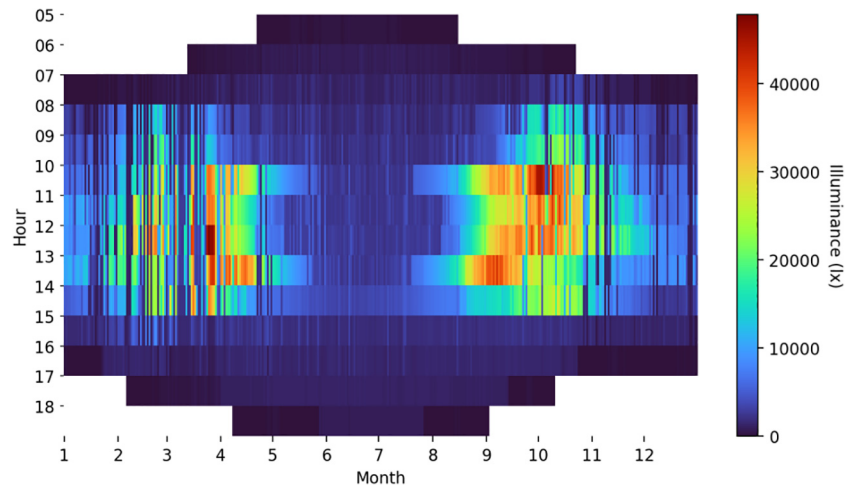
Fig. 4. Workplane illuminance (lx) data for each hour (y-axis) and day (x-axis) of the year. Hourly data were generated from the three-phase simulation. Source: LBNL.
